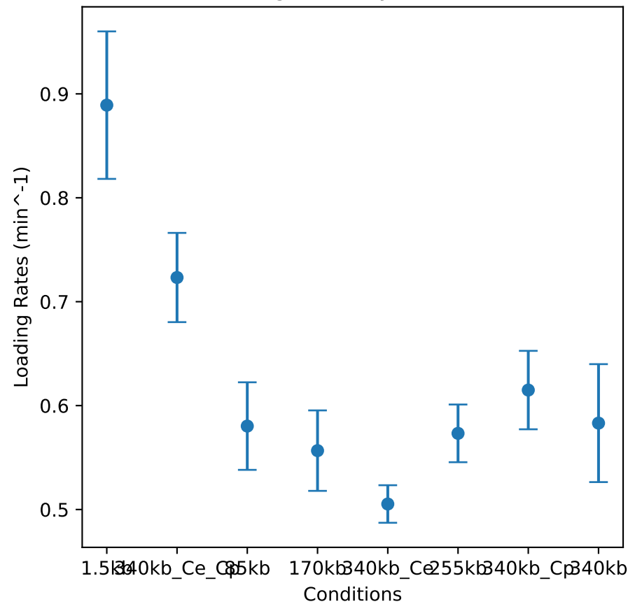
Loading Rates by Condition
