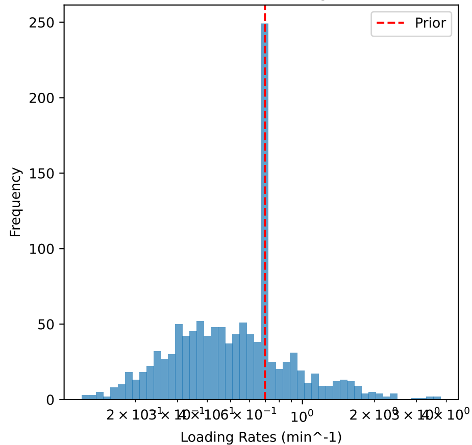
Distribution of Loading Rates
