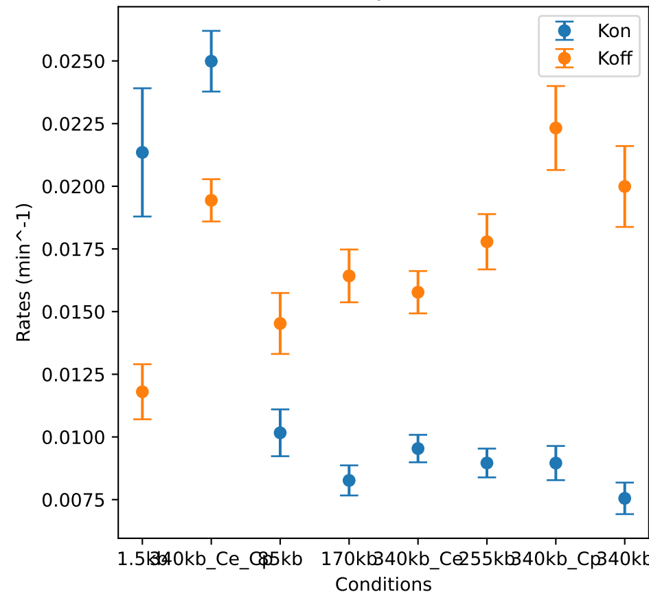
Koff/kon by Condition
