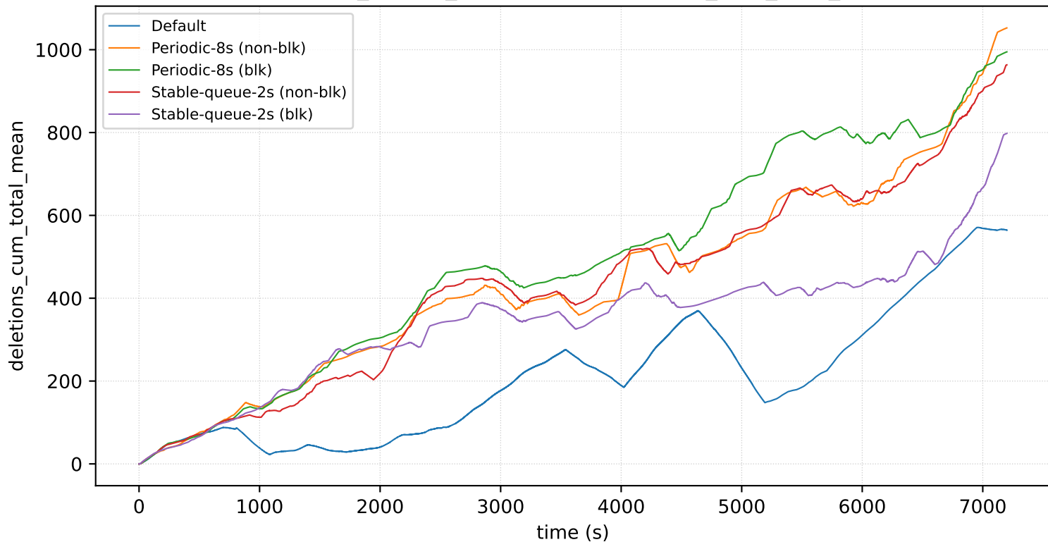
nodes=16_prio=1_arrival=16s: deletions_cum_total_mean
