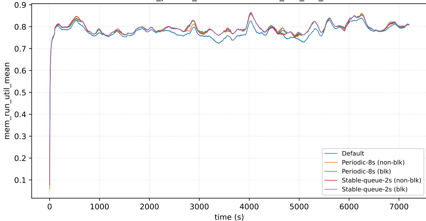
nodes=16_prio=1_arrival=16s: mem_run_util_mean
