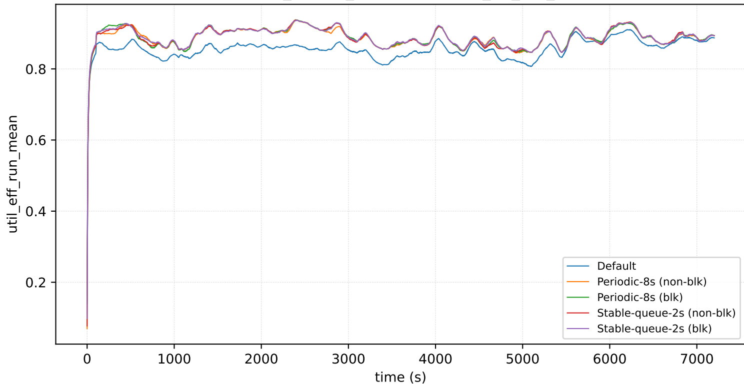
nodes=16_prio=1_arrival=16s: util_eff_run_mean
