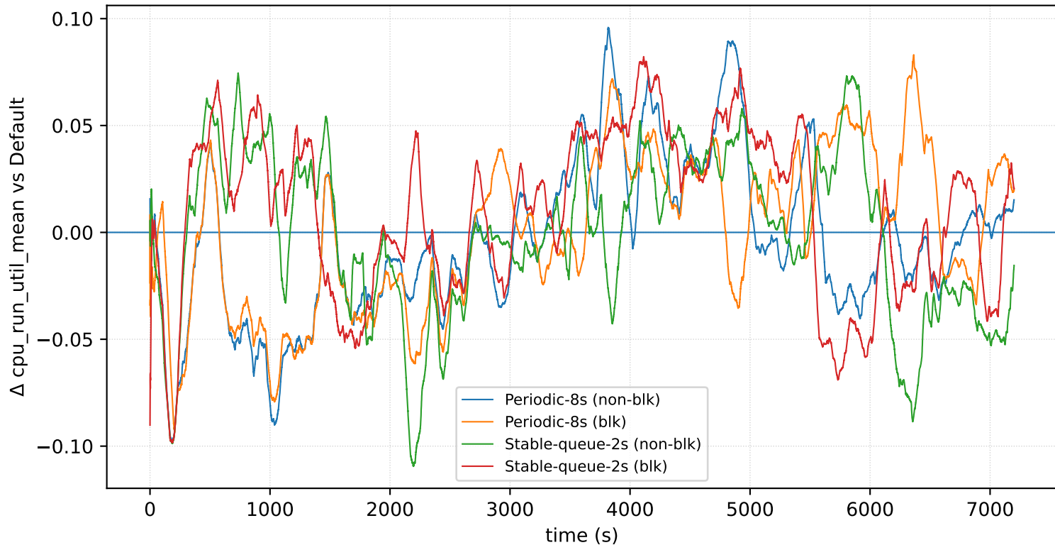
nodes=16_prio=1_arrival=4s: \Delta cpu_run_util_mean
