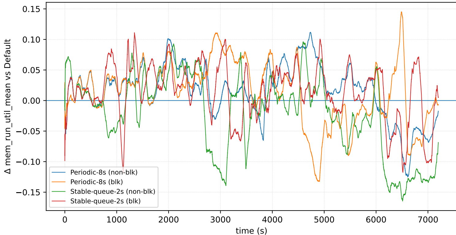
nodes=16_prio=1_arrival=4s: \Delta mem_run_util_mean
