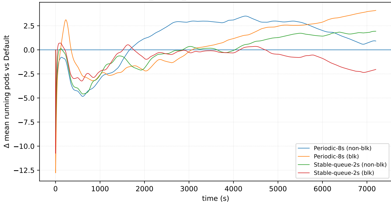
nodes=16_prio=1_arrival=8s: \Delta mean running pods
