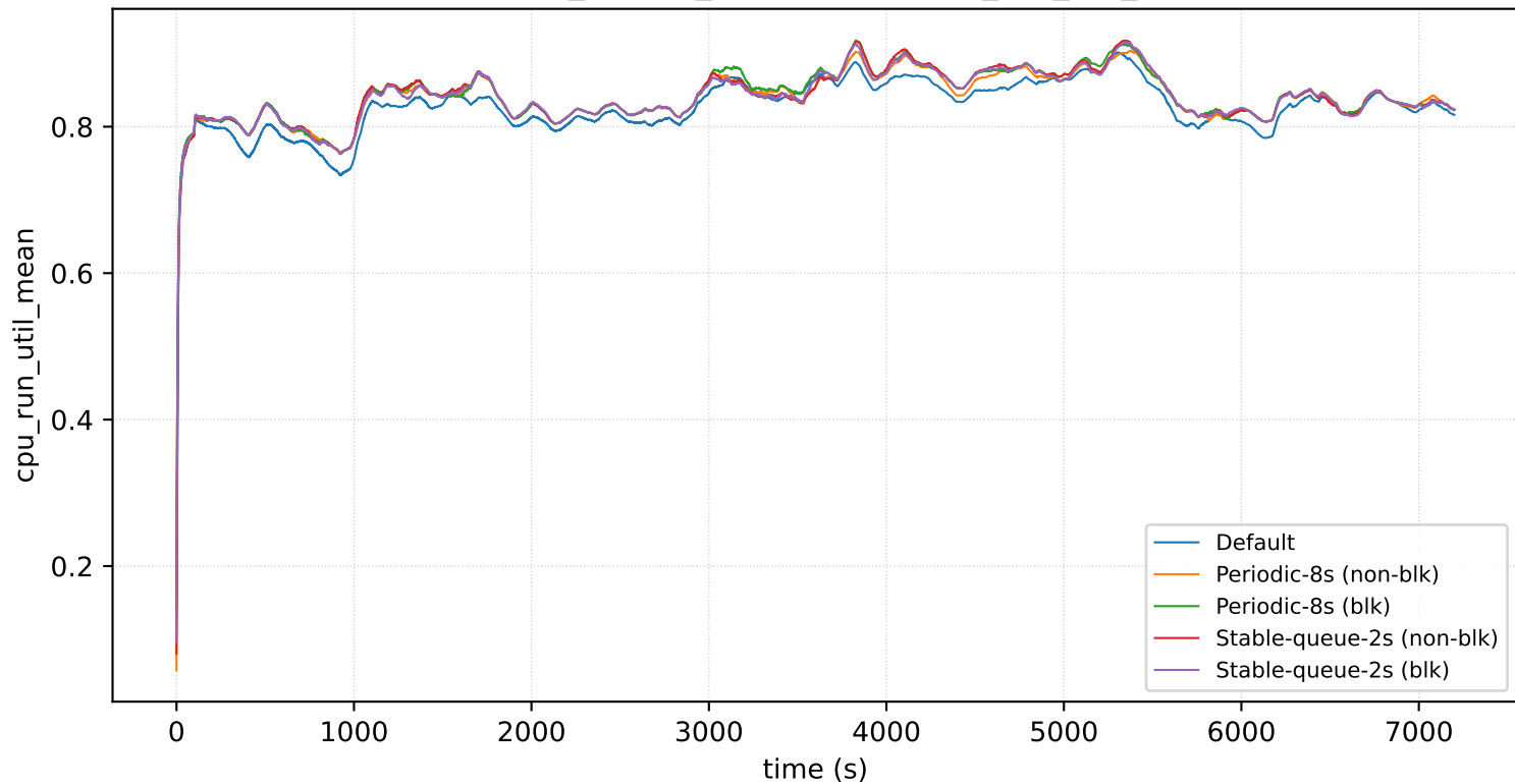
nodes=16_prio=4_arrival=16s: cpu_run_util_mean
