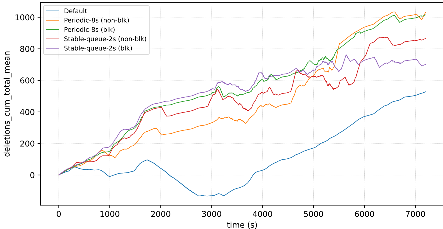
nodes=16_prio=4_arrival=16s: deletions_cum_total_mean
