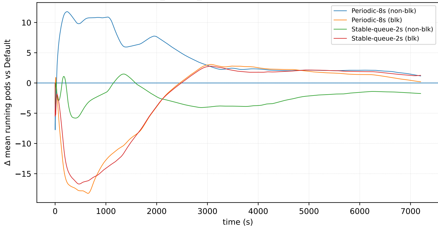
nodes=16_prio=4_arrival=16s: \Delta mean running pods
