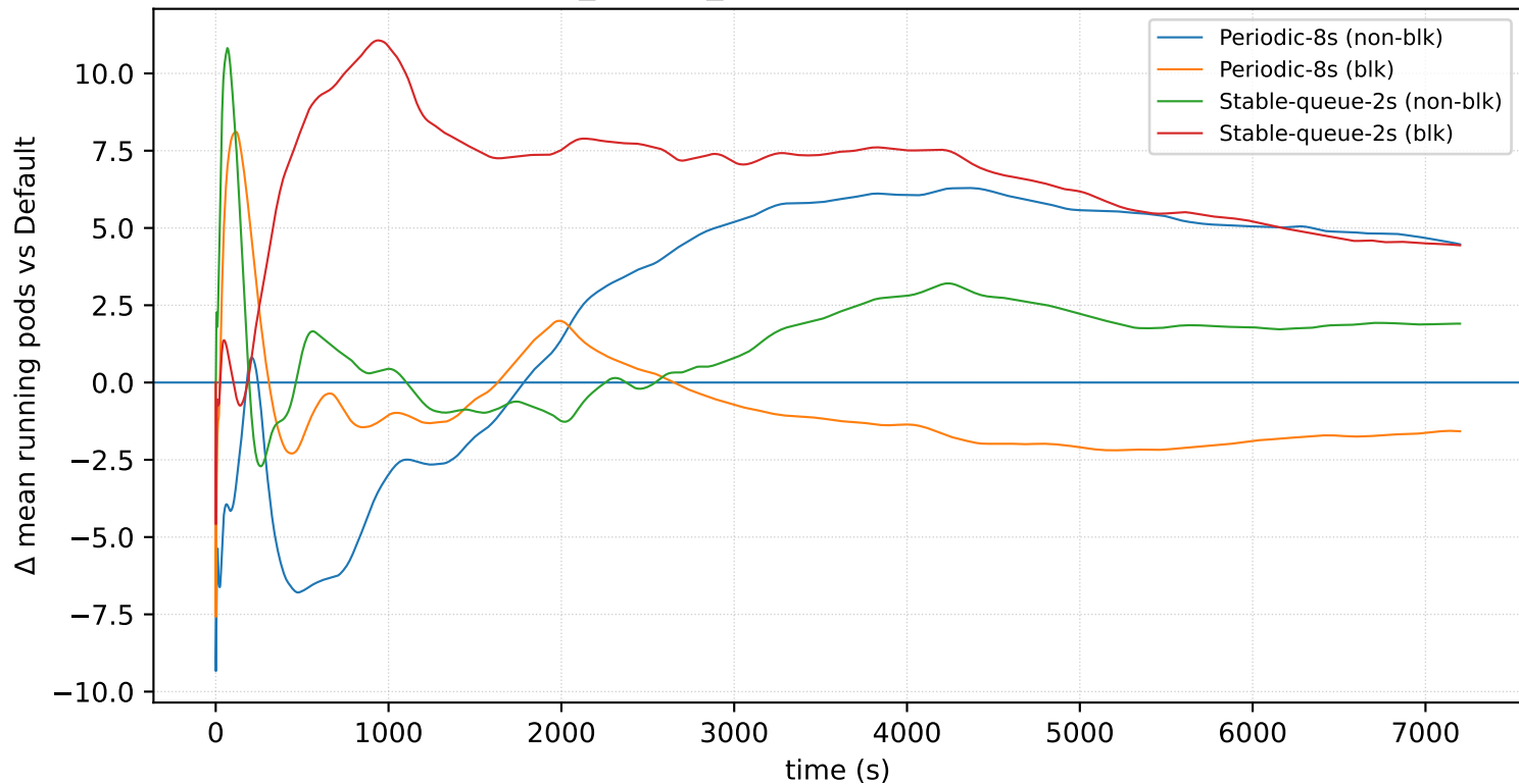
nodes=16_prio=4_arrival=4s: \Delta mean running pods
