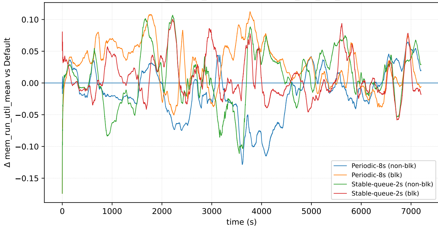
nodes=16_prio=4_arrival=8s: \Delta mem_run_util_mean
