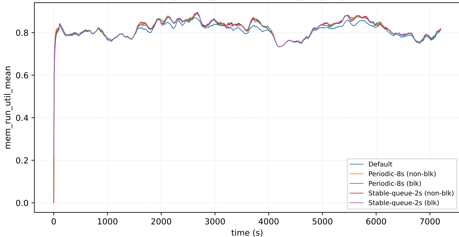
nodes=16_prio=4_arrival=8s: mem_run_util_mean
