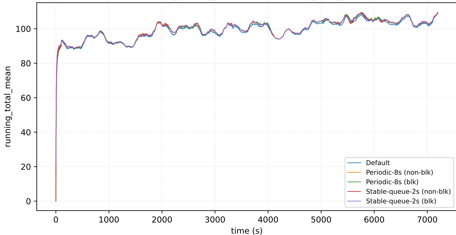
nodes=16_prio=4_arrival=8s: running_total_mean
