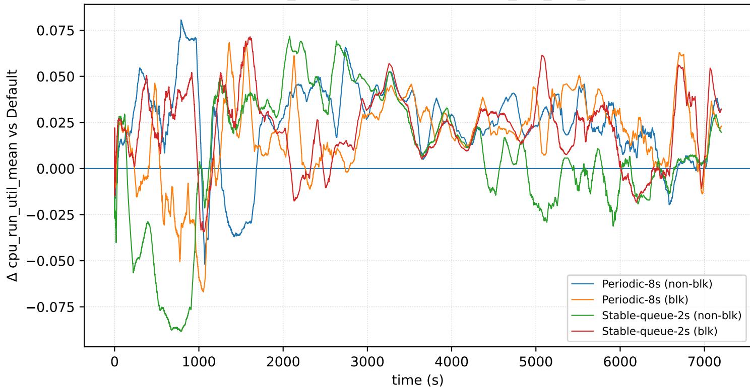
nodes=32_prio=1_arrival=16s: \Delta cpu_run_util_mean
