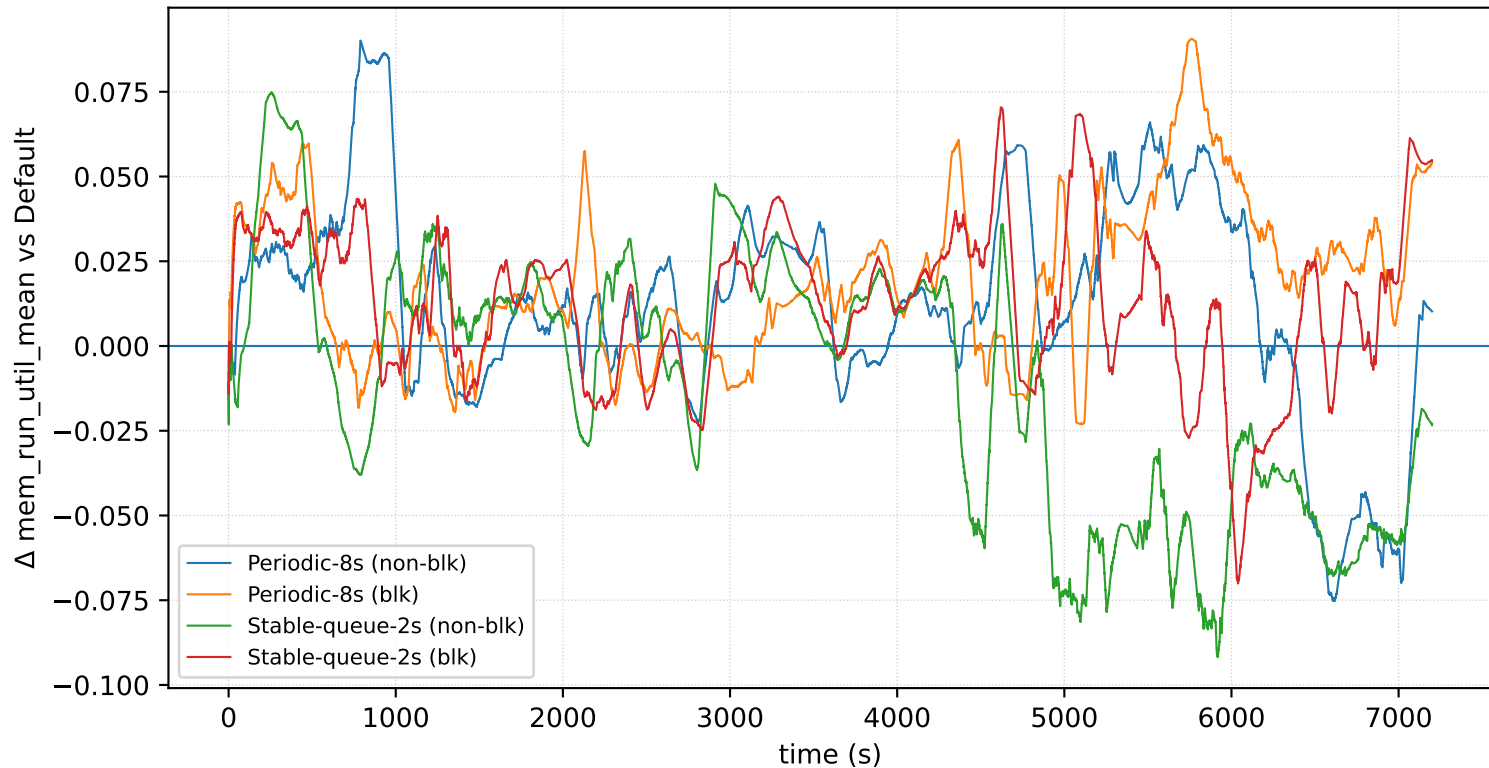
nodes=32_prio=1_arrival=16s: \Delta mem_run_util_mean
