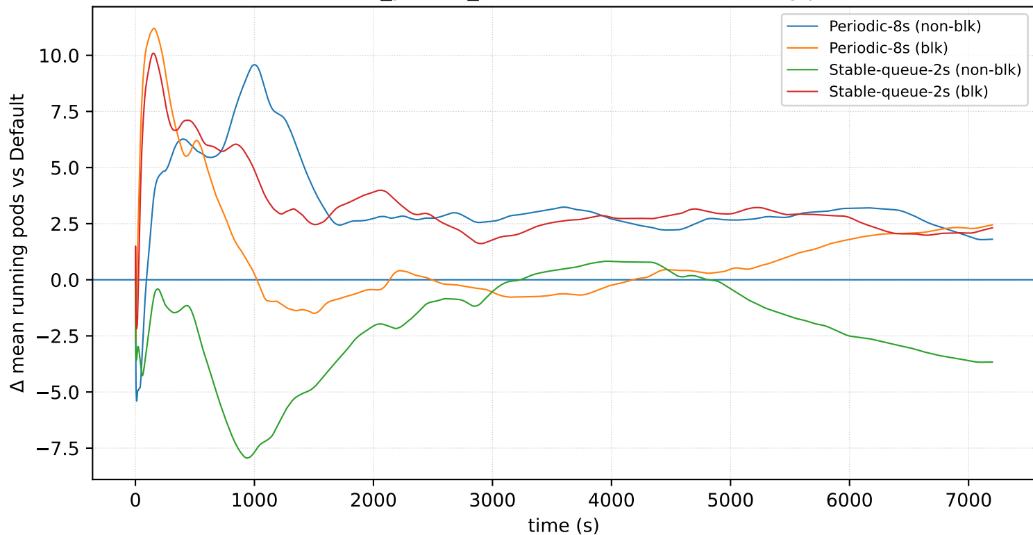
nodes=32_prio=1_arrival=16s: \Delta mean running pods
