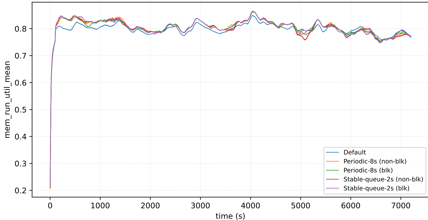
nodes=32_prio=1_arrival=16s: mem_run_util_mean
