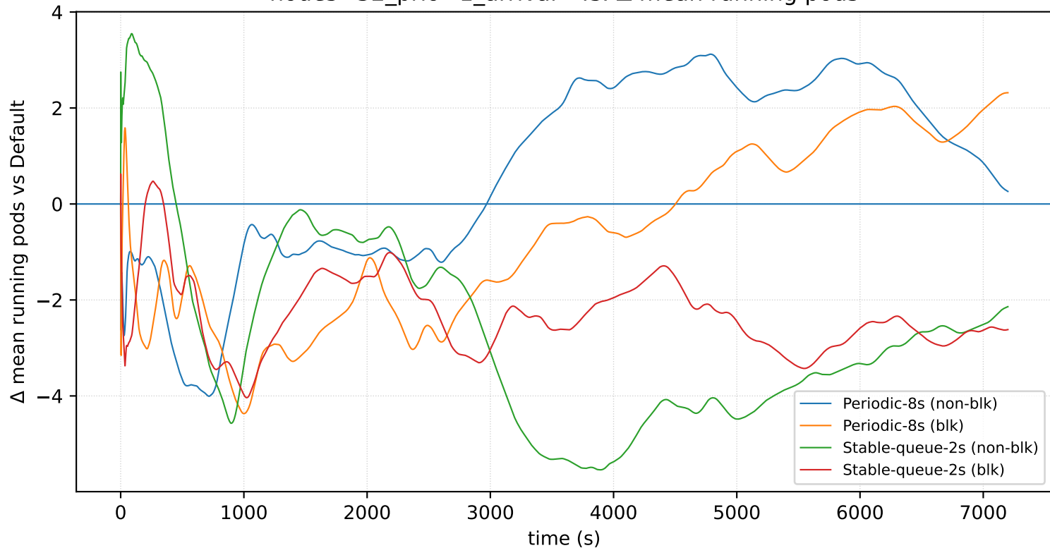
nodes=32_prio=1_arrival=4s: \Delta mean running pods
