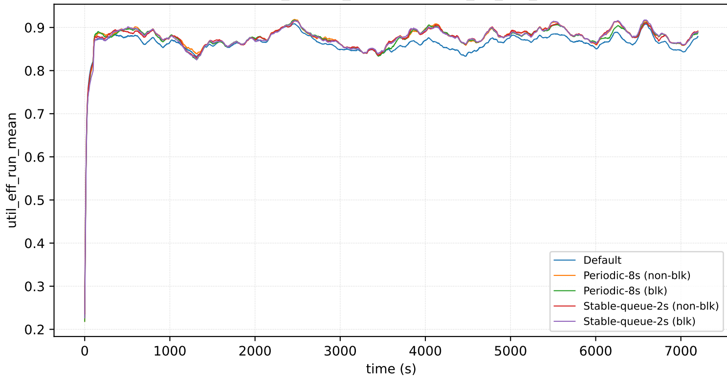
nodes=32_prio=1_arrival=4s: util_eff_run_mean
