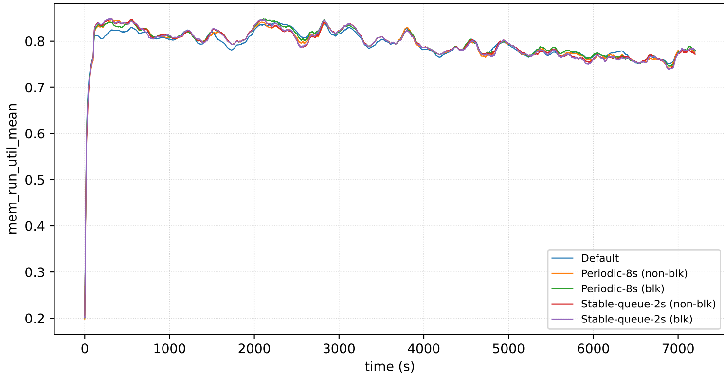
nodes=32_prio=1_arrival=8s: mem_run_util_mean
