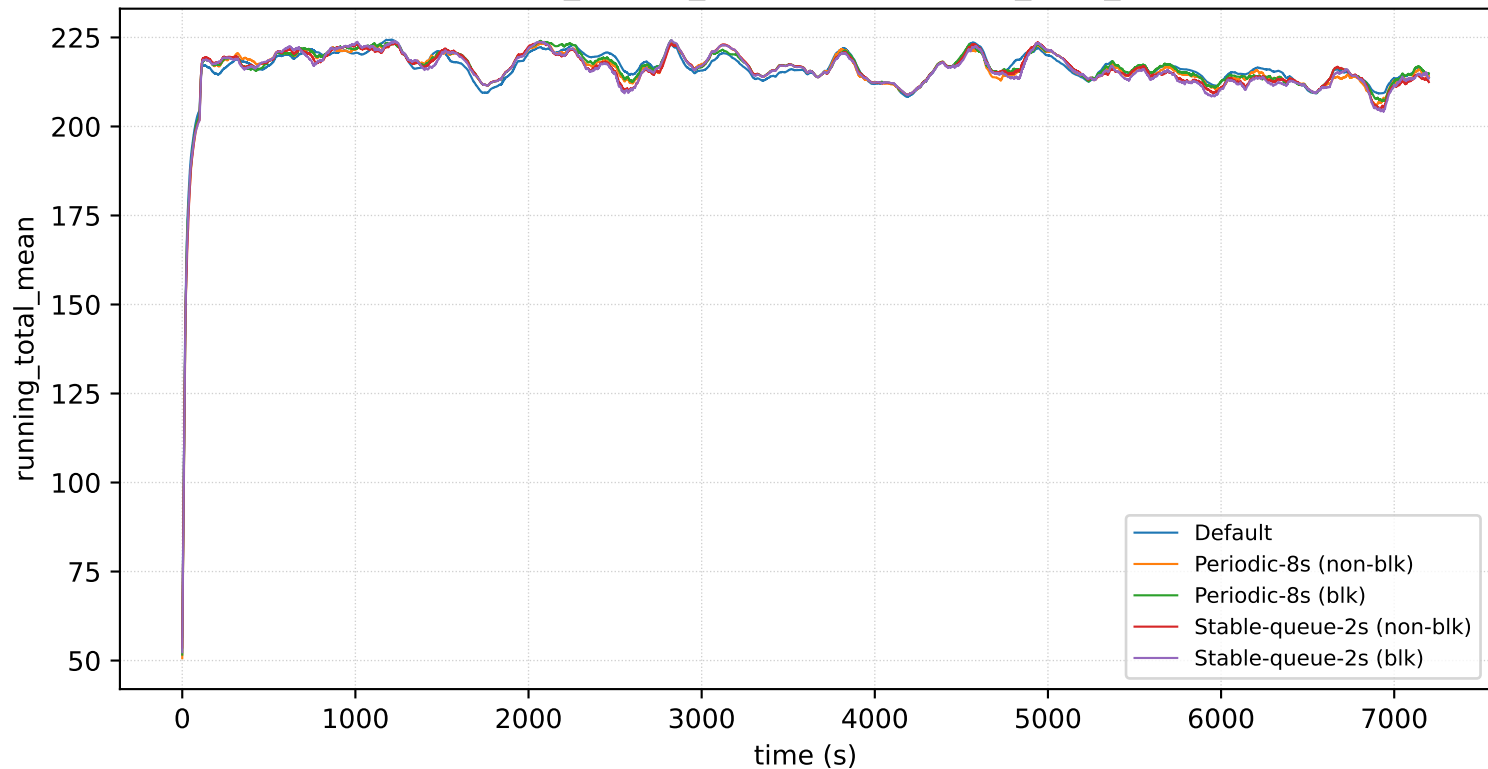
nodes=32_prio=1_arrival=8s: running_total_mean
