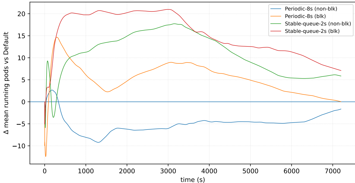
nodes=32_prio=4_arrival=16s: \Delta mean running pods
