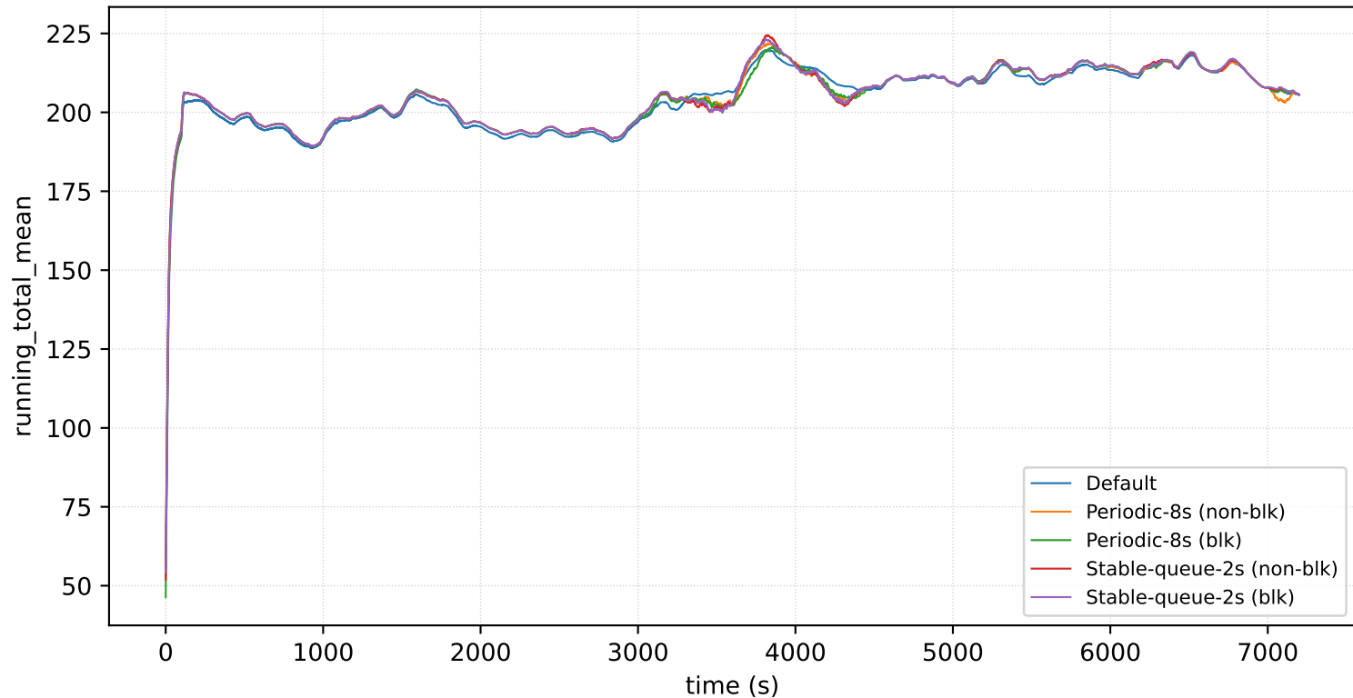
nodes=32_prio=4_arrival=16s: running_total_mean
