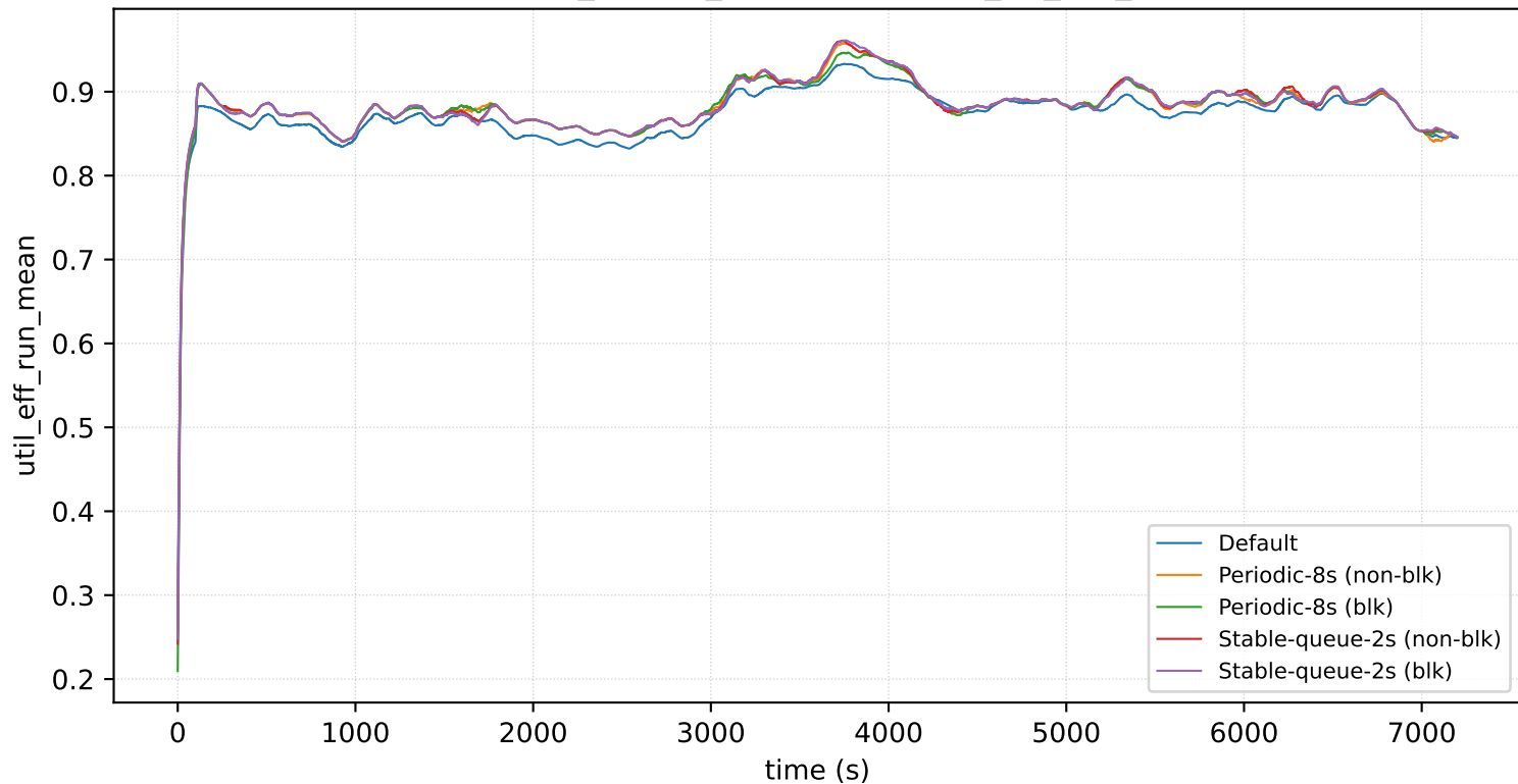
nodes=32_prio=4_arrival=16s: util_eff_run_mean
