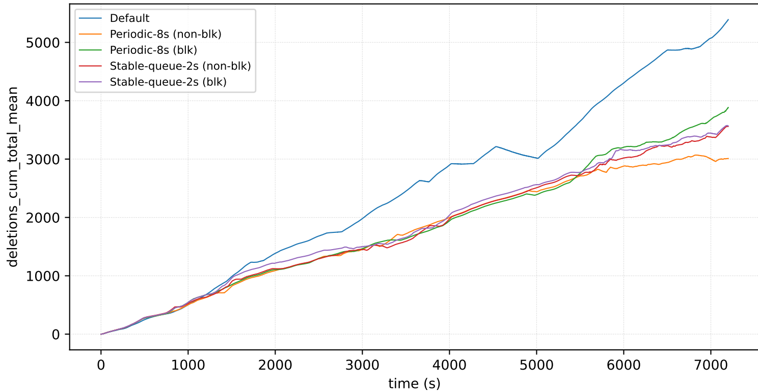
nodes=32_prio=4_arrival=4s: deletions_cum_total_mean
