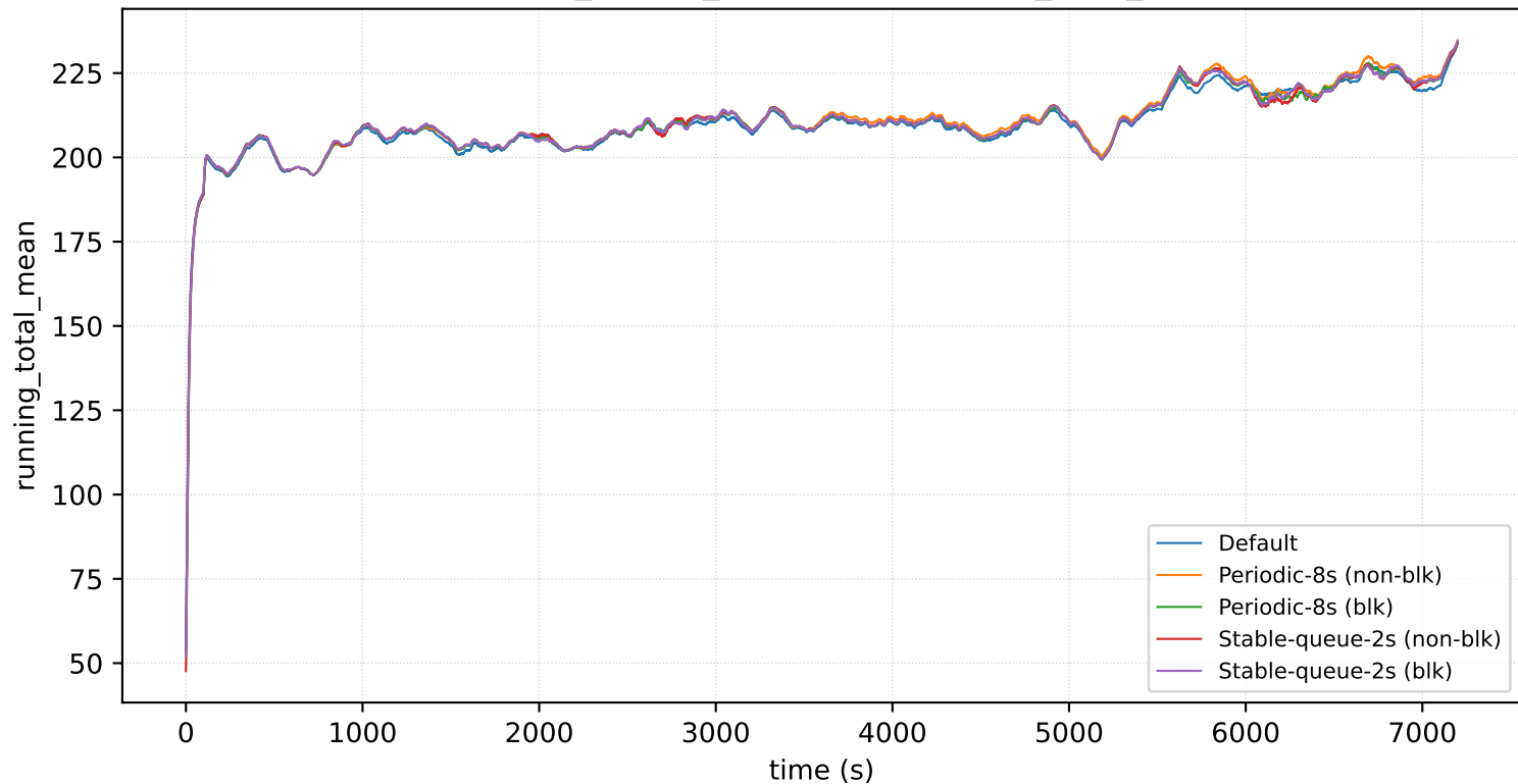
nodes=32_prio=4_arrival=4s: running_total_mean
