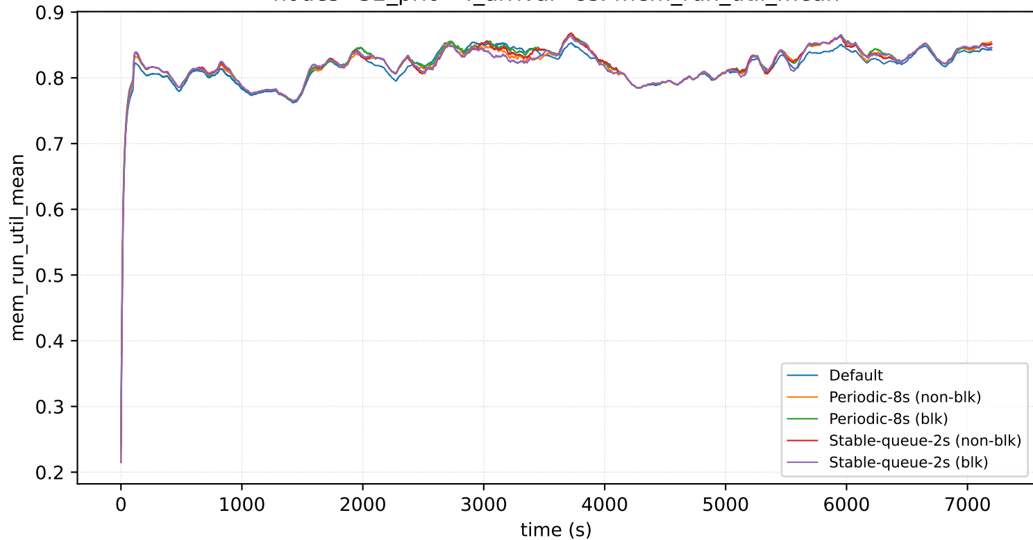
nodes=32_prio=4_arrival=8s: mem_run_util_mean
