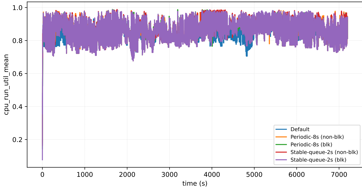
nodes=16_prio=1_arrival=4s: cpu_run_util_mean
