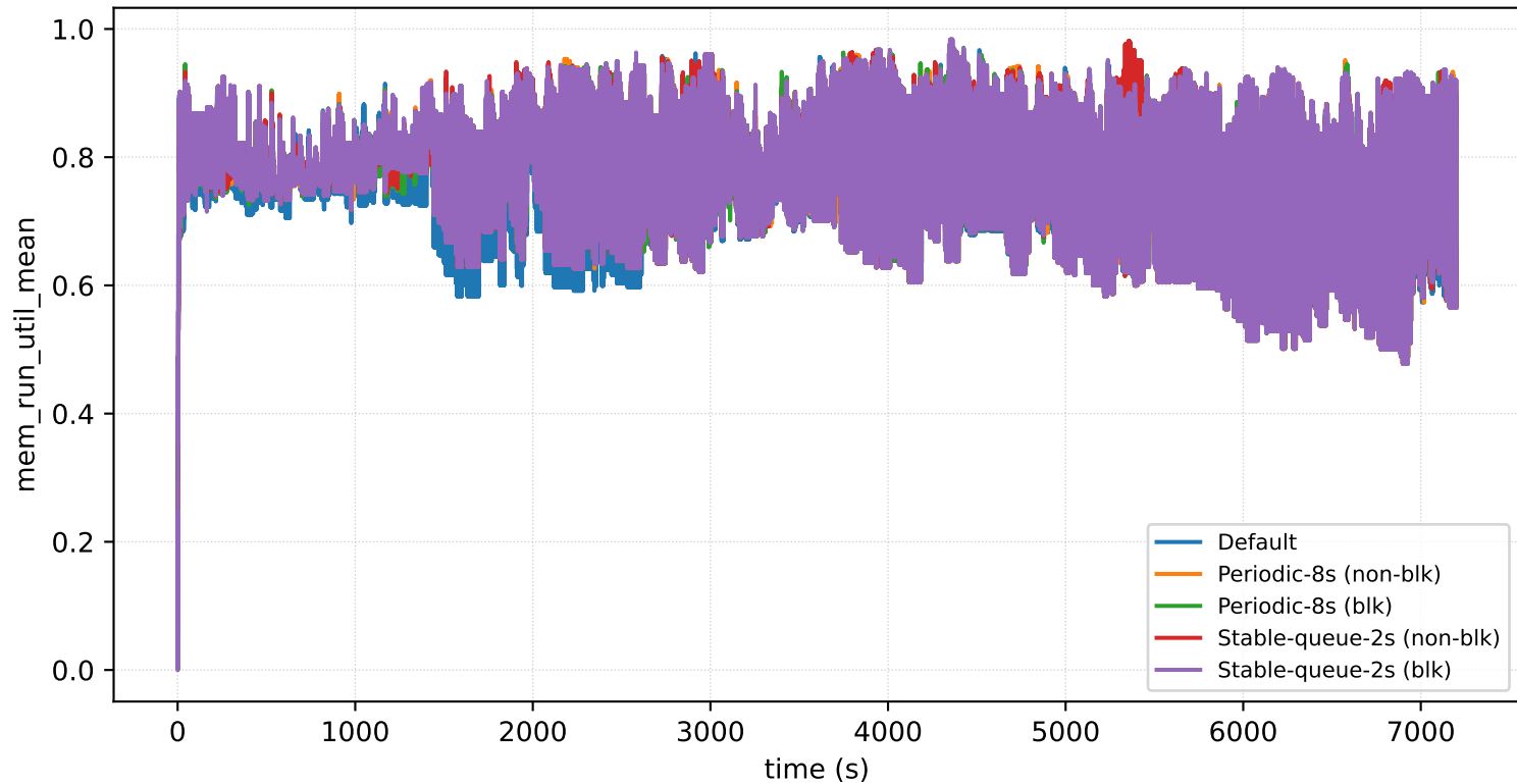
nodes=16_prio=1_arrival=8s: mem_run_util_mean
