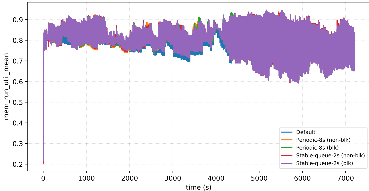
nodes=32_prio=1_arrival=16s: mem_run_util_mean
