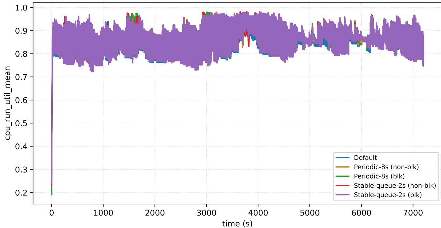
nodes=32_prio=4_arrival=16s: cpu_run_util_mean
