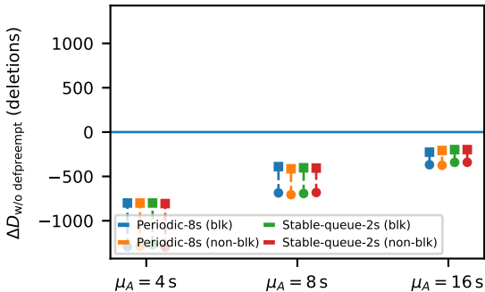
\Delta D_{\text{w/o defpreempt}} (count) vs \mu_A (kmax=4)
