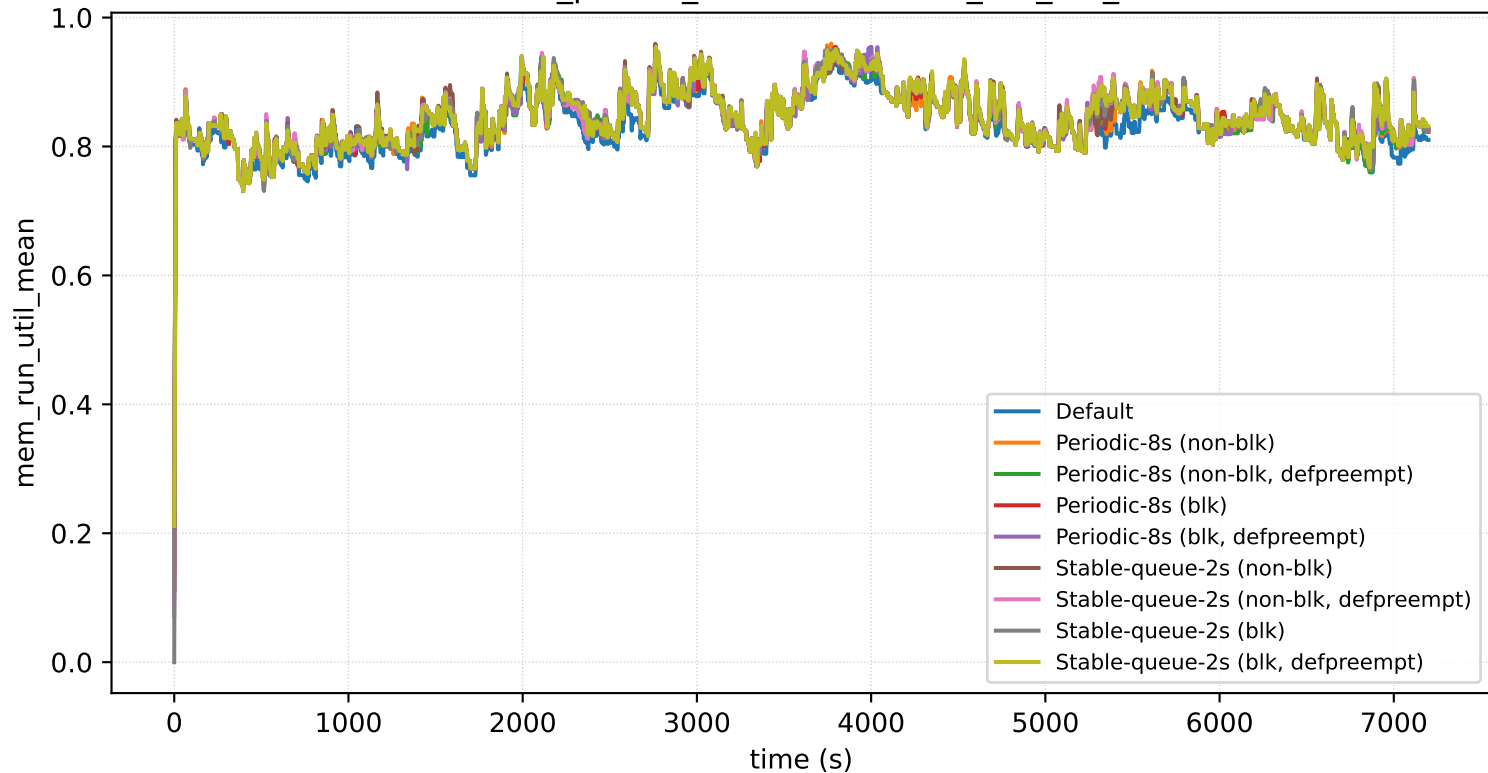
nodes=16_prio=1_arrival=8s: mem_run_util_mean
