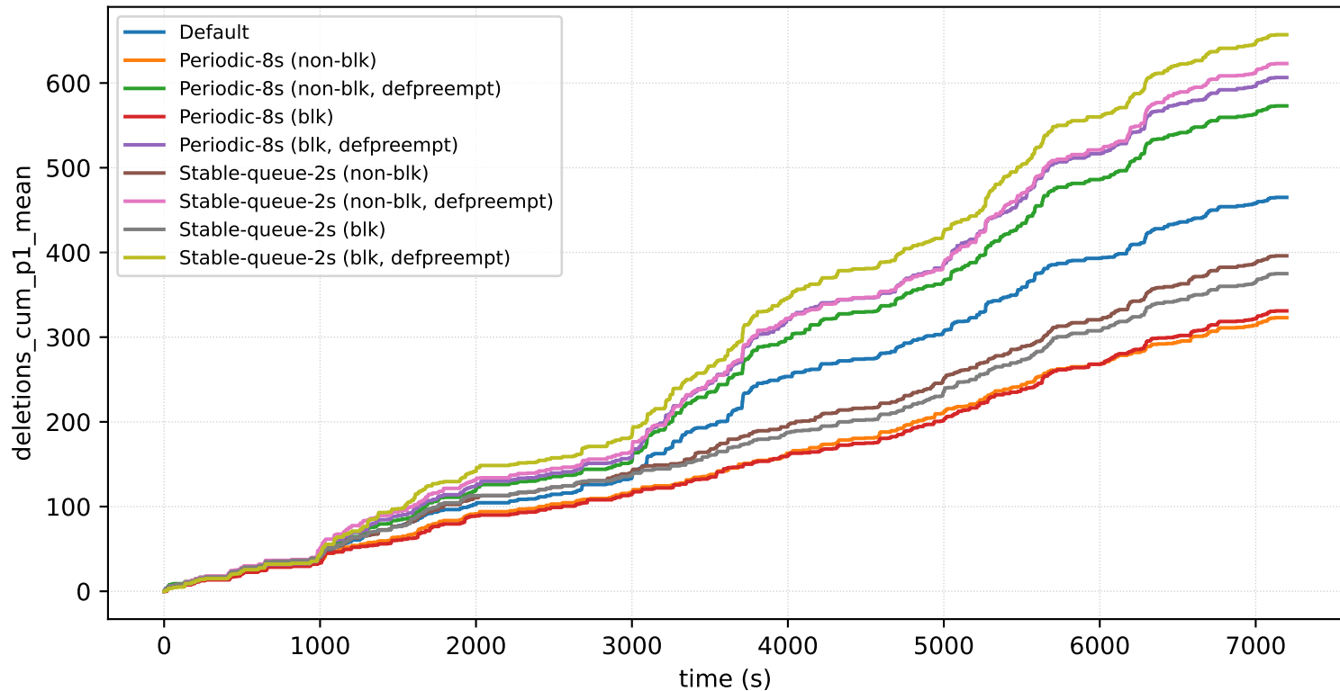
nodes=16_prio=4_arrival=16s: deletions_cum_p1_mean
