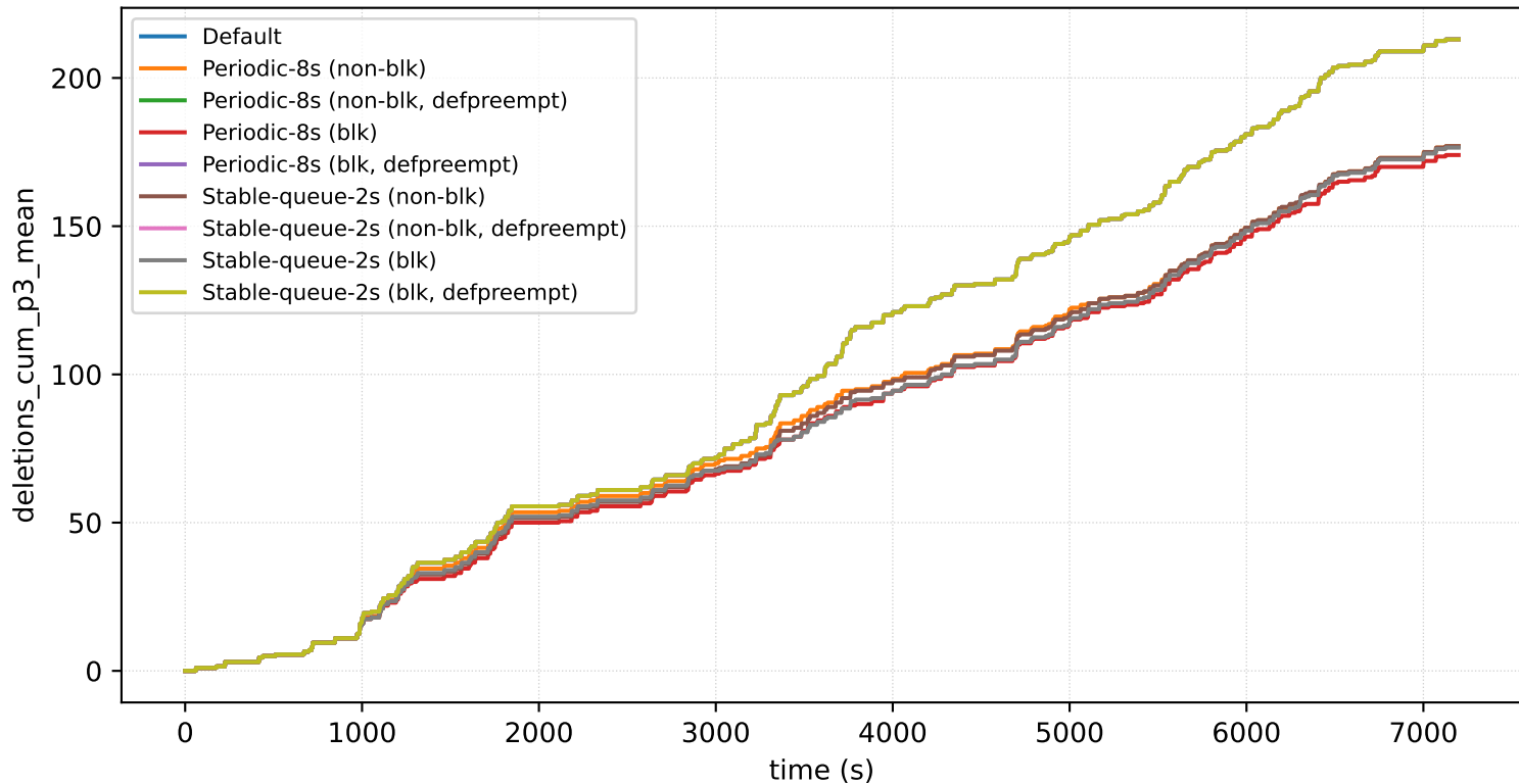
nodes=16_prio=4_arrival=16s: deletions_cum_p3_mean
