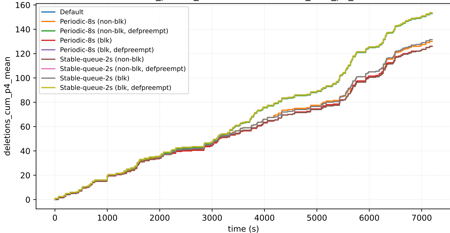
nodes=16_prio=4_arrival=16s: deletions_cum_p4_mean
