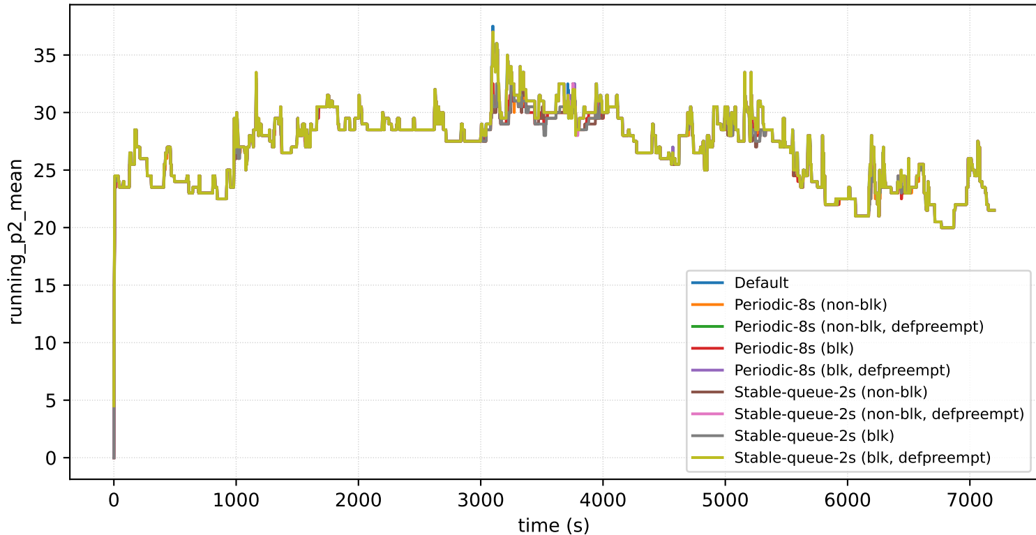
nodes=16_prio=4_arrival=16s: running_p2_mean
