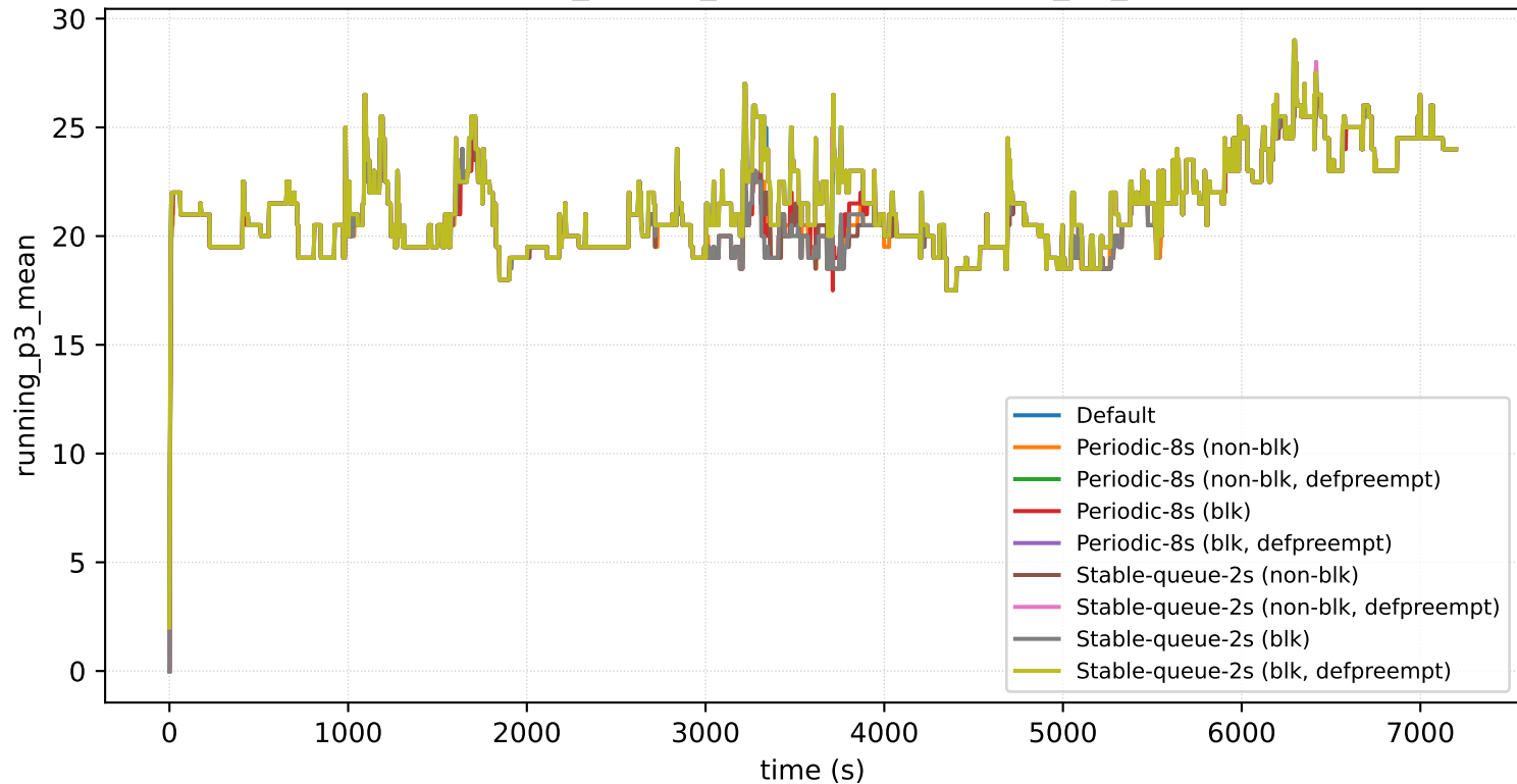
nodes=16_prio=4_arrival=16s: running_p3_mean
