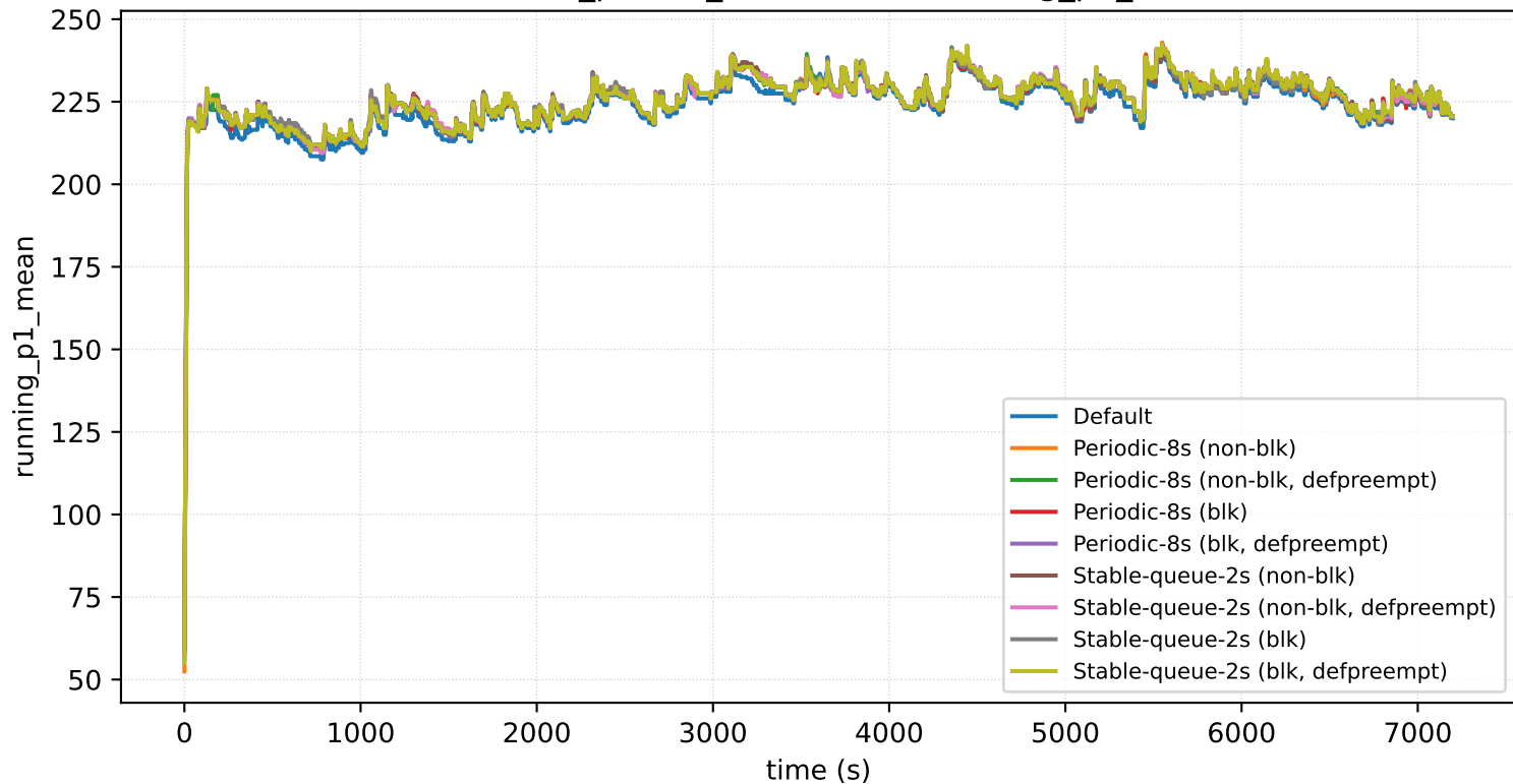
nodes=32_prio=1_arrival=16s: running_p1_mean
