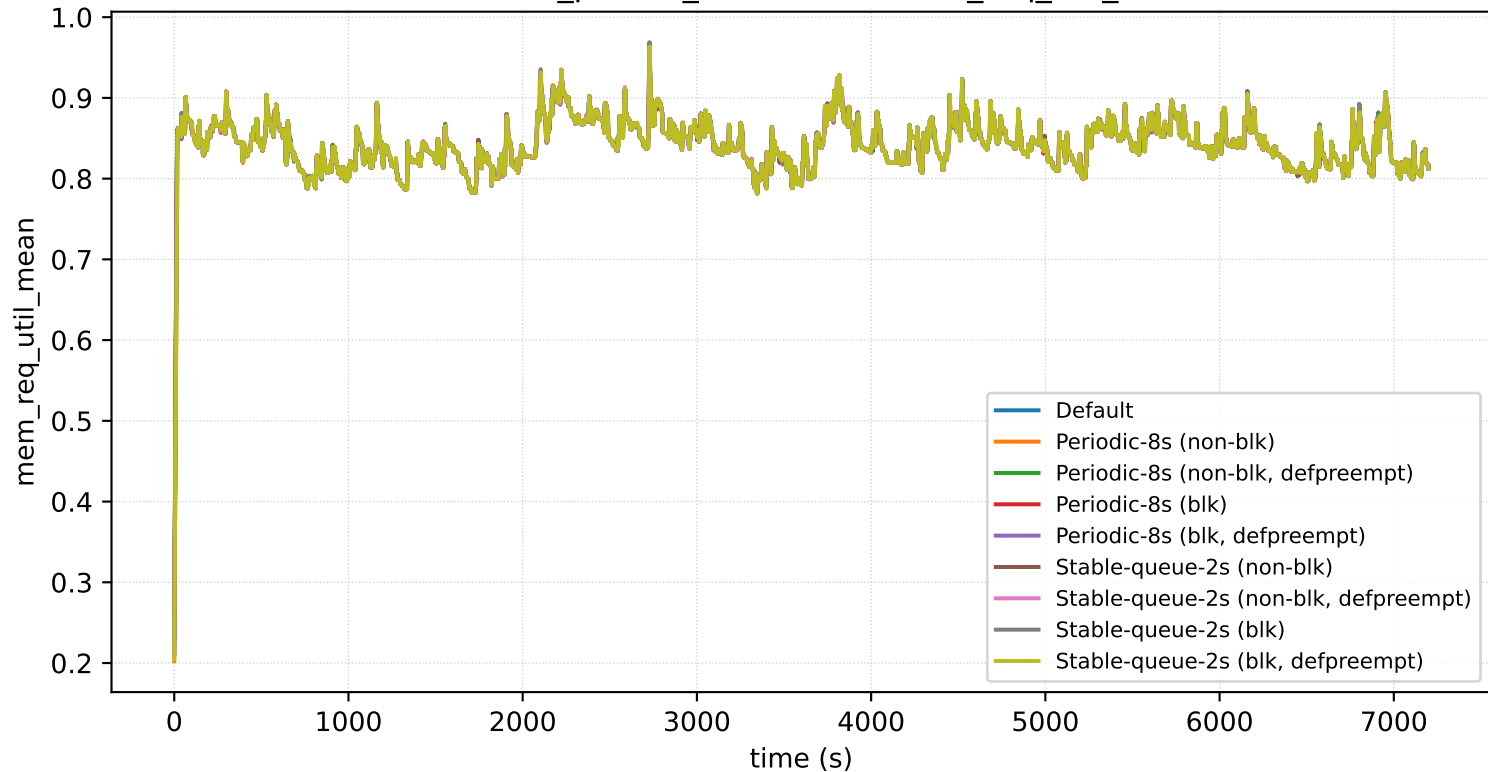
nodes=32_prio=1_arrival=8s: mem_req_util_mean
