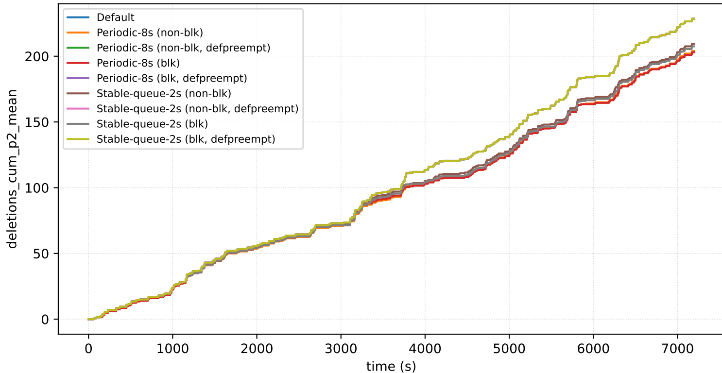
nodes=32_prio=4_arrival=16s: deletions_cum_p2_mean
