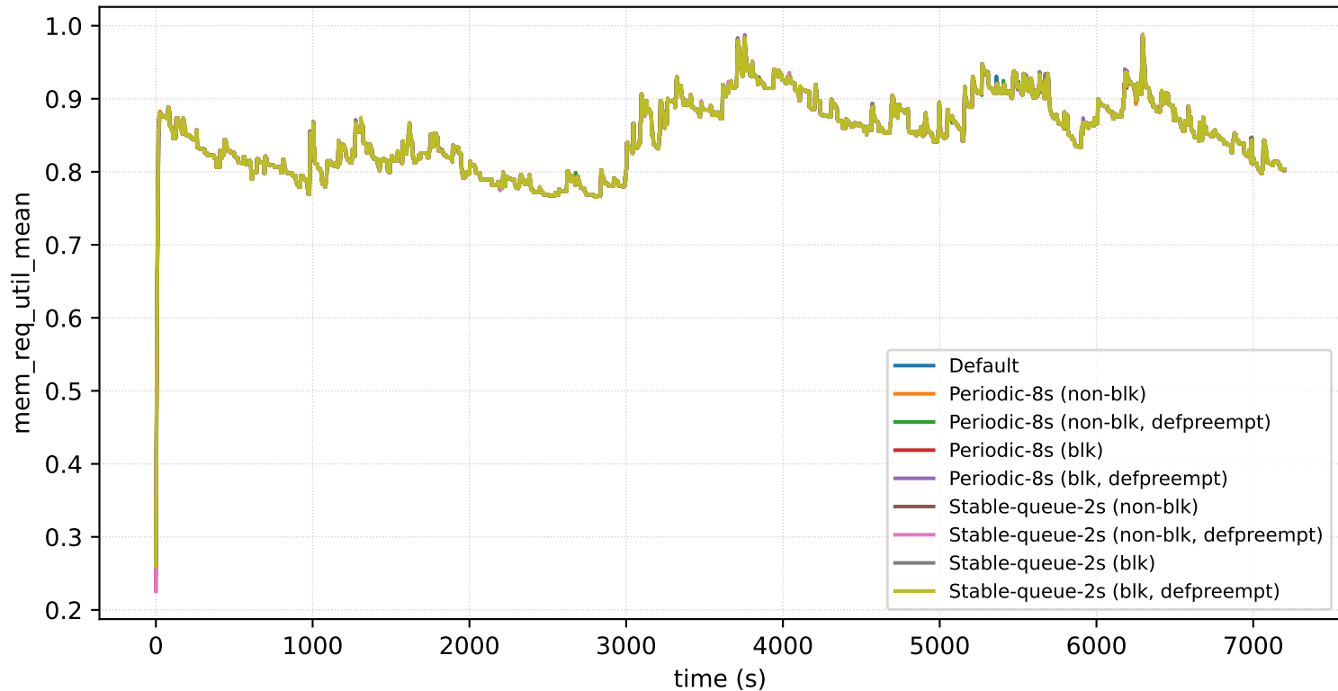
nodes=32_prio=4_arrival=16s: mem_req_util_mean
