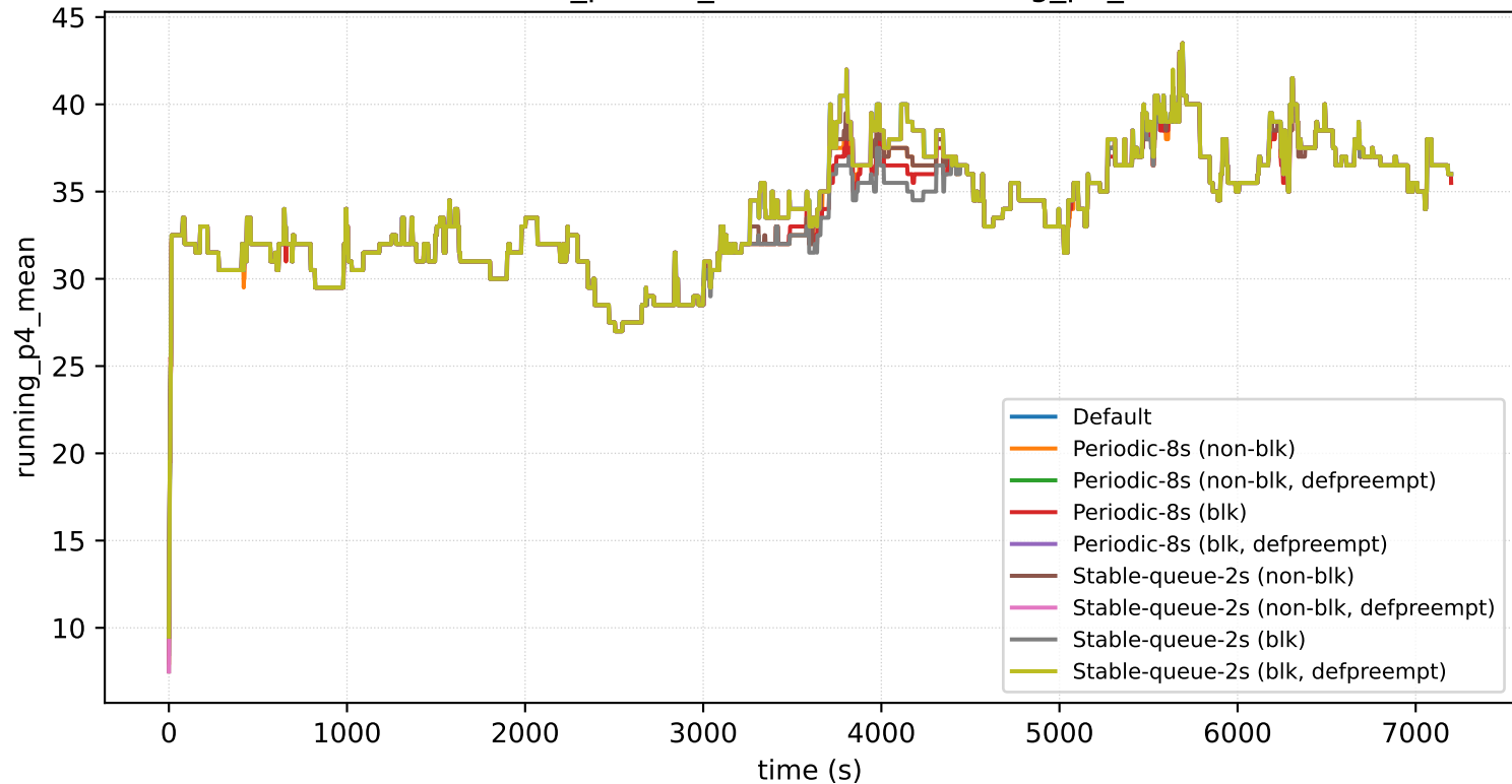
nodes=32_prio=4_arrival=16s: running_p4_mean
