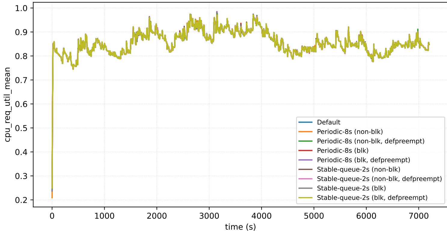
nodes=32_prio=4_arrival=8s: cpu_req_util_mean
