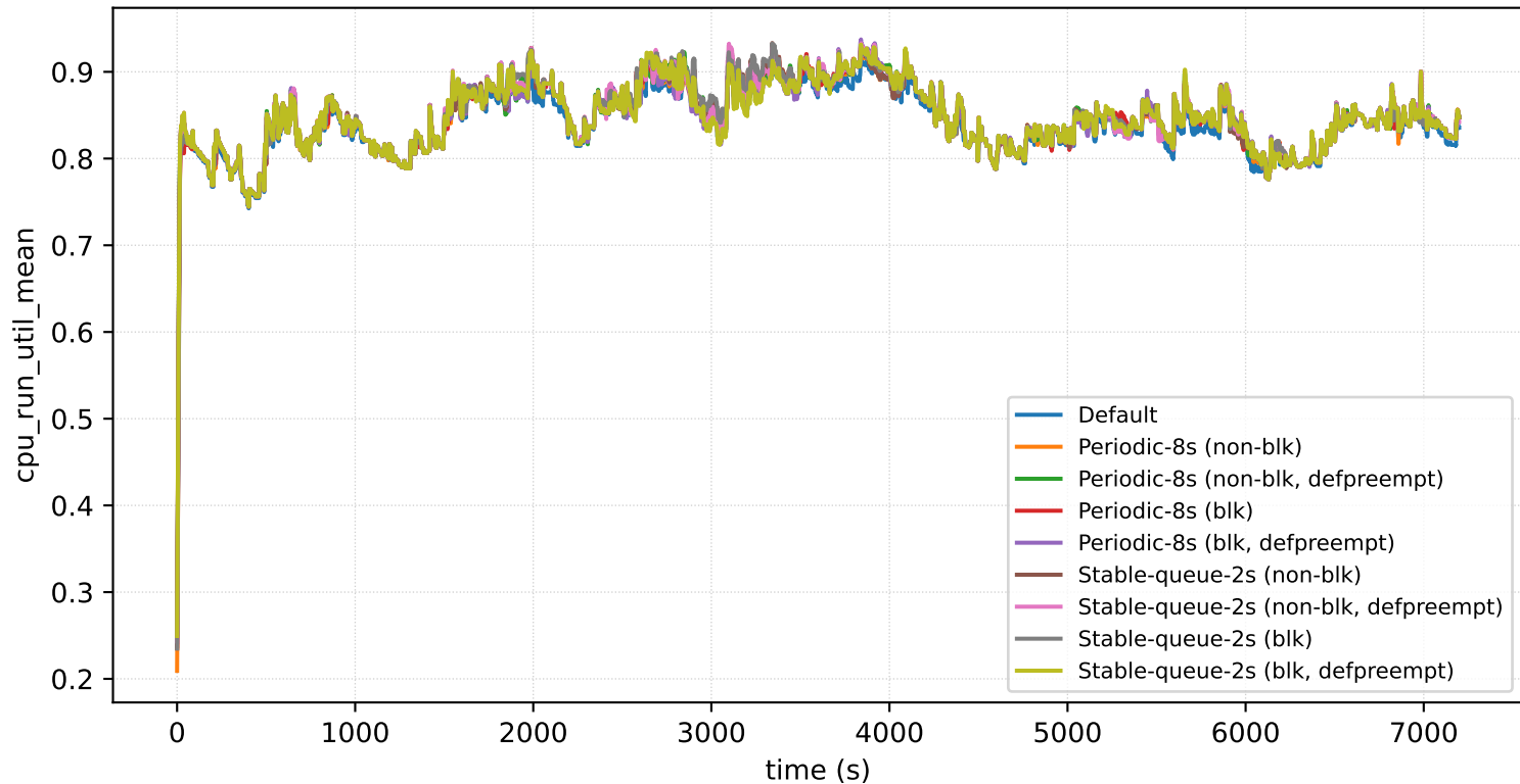
nodes=32_prio=4_arrival=8s: cpu_run_util_mean
