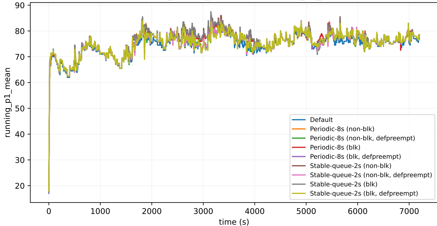
nodes=32_prio=4_arrival=8s: running_p1_mean
