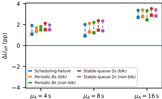
\Delta U_{\text{eff}} vs \mu_A (kmax=1)
