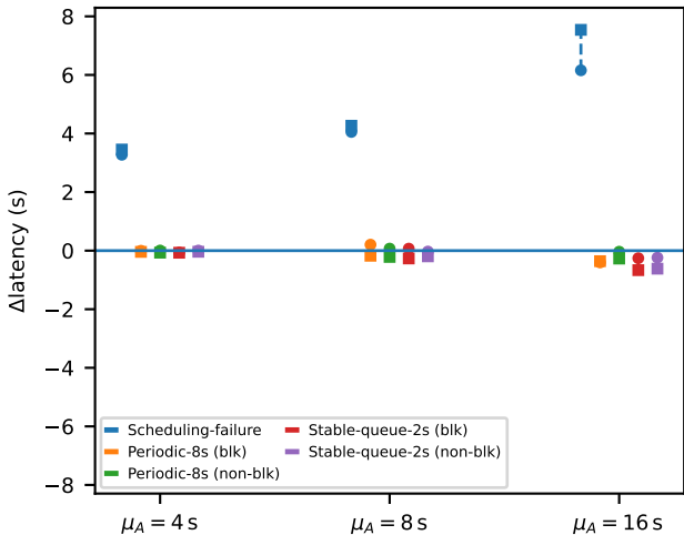
\Delta\text{latency}_{\text{total}} (s) vs \mu_A (kmax=4)
