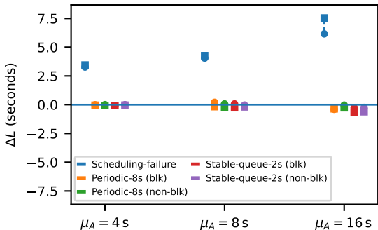
\Delta L vs \mu_A (kmax=4)
